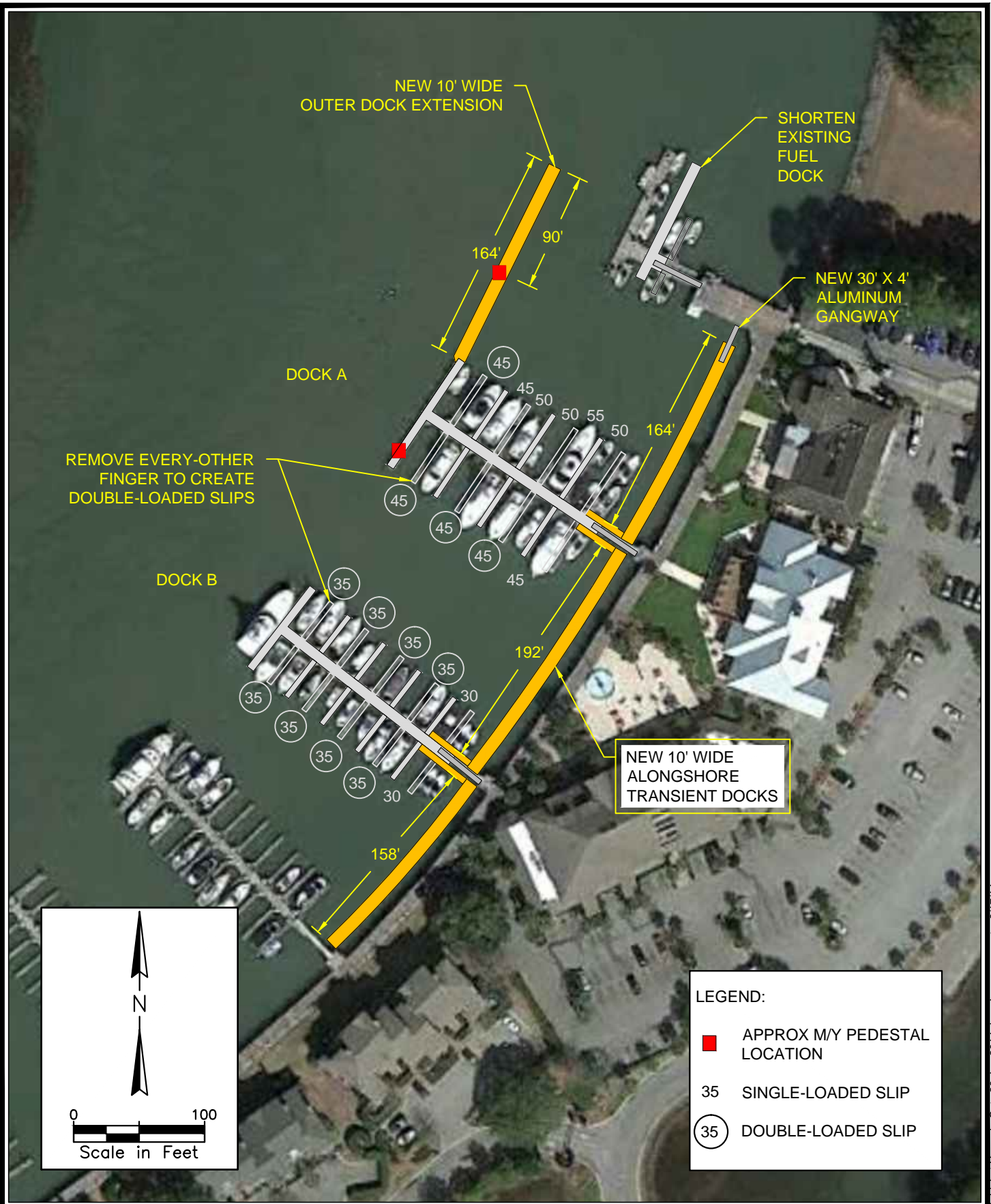
FIGURE 2 - PROPOSED IMPROVEMENTS Bohicket Marina Boating Infrastructure Grant Application FY 2015 - Tier 2
